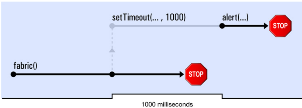
Figure 5.5. Calling setTimeout schedules a task to be run after a delay
